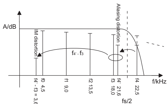
Figure 5, IM distortion example
